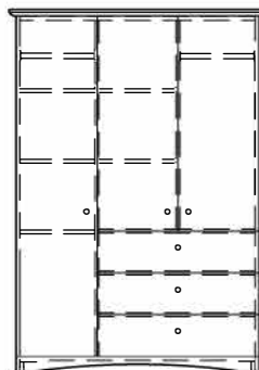
MODEL HCAM48-126-A-K (finish)
