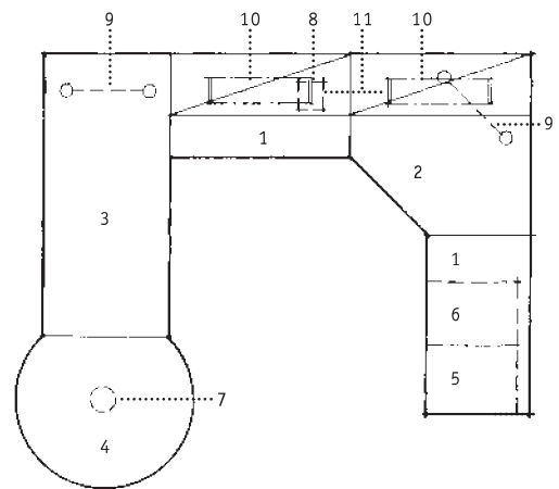
FLAT TIRE WORKSTATION 96" X 120"
